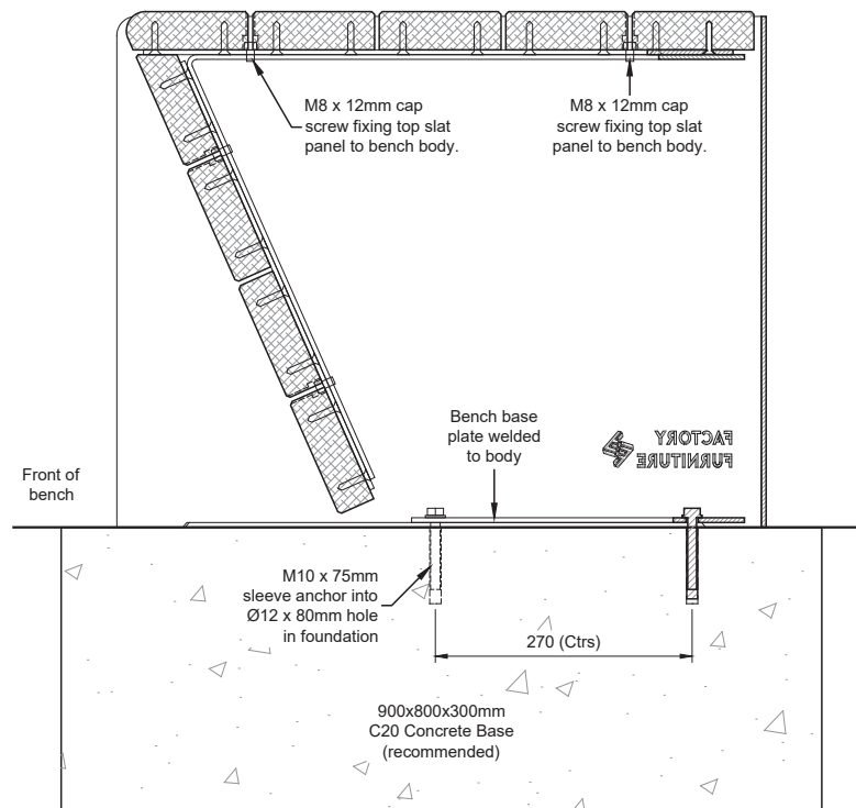
X-Section Thro' Bench
