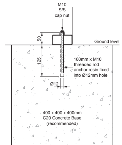
Base fix detail (showing bench)
