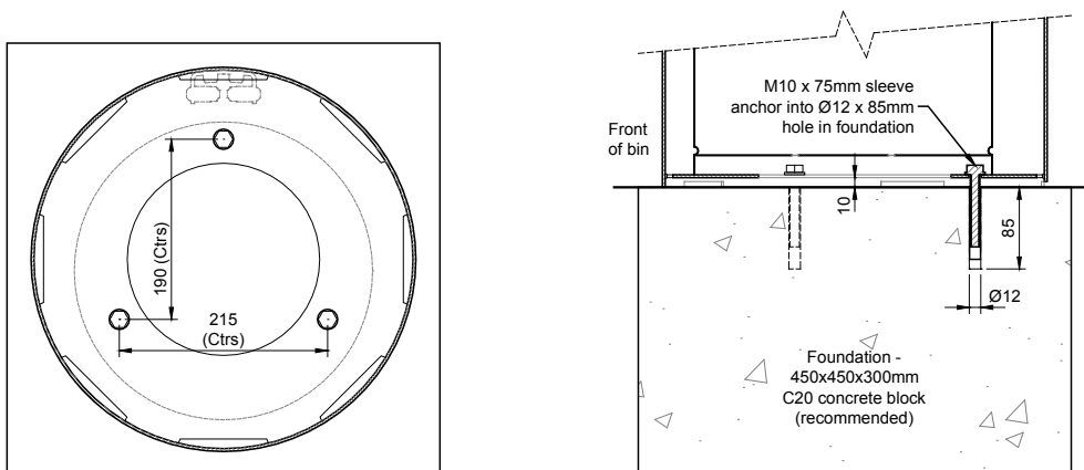
Fixing detail
