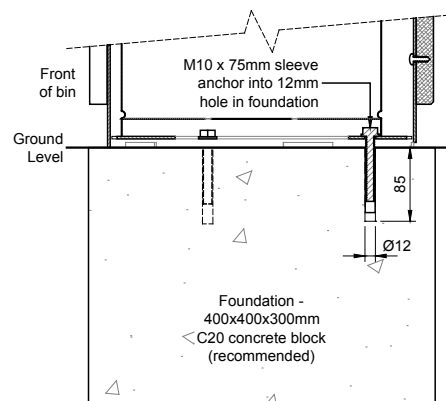
Fixing detail
