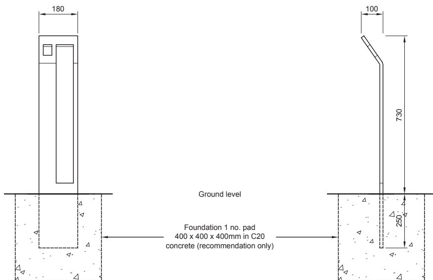
Bike Stand ( Sub-surface Fix Only )
